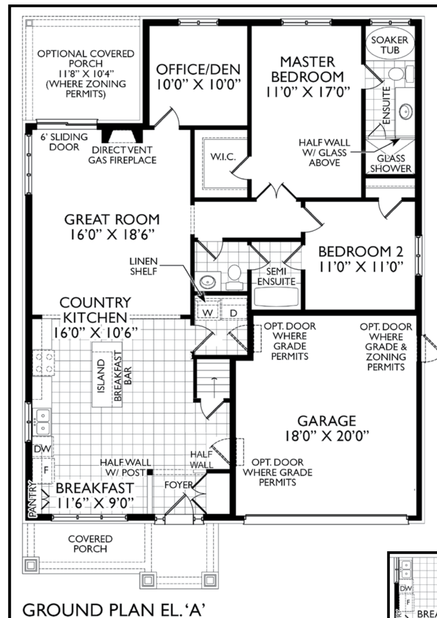
Elevation A - 1,517 square feet (1,600 with extended garage)
