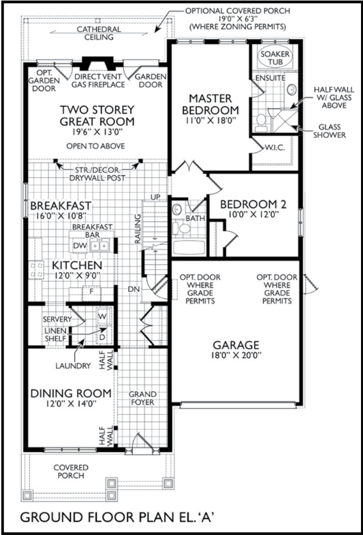
Elevation A - 1,773 square feet (2,474 with loft) (2,480 with extended garage)
