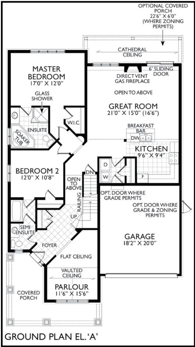
Elevation A - 1,653 square feet (2,137 with loft) (2,218 with extended garage)
